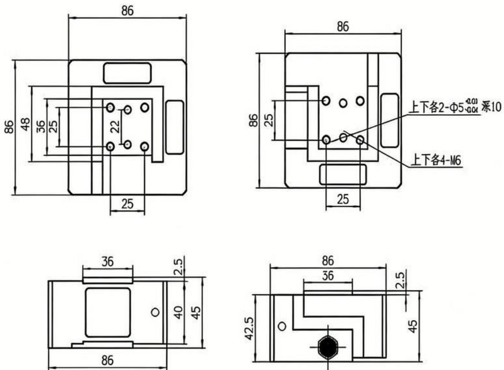
MLC5086SF3-SIZE
