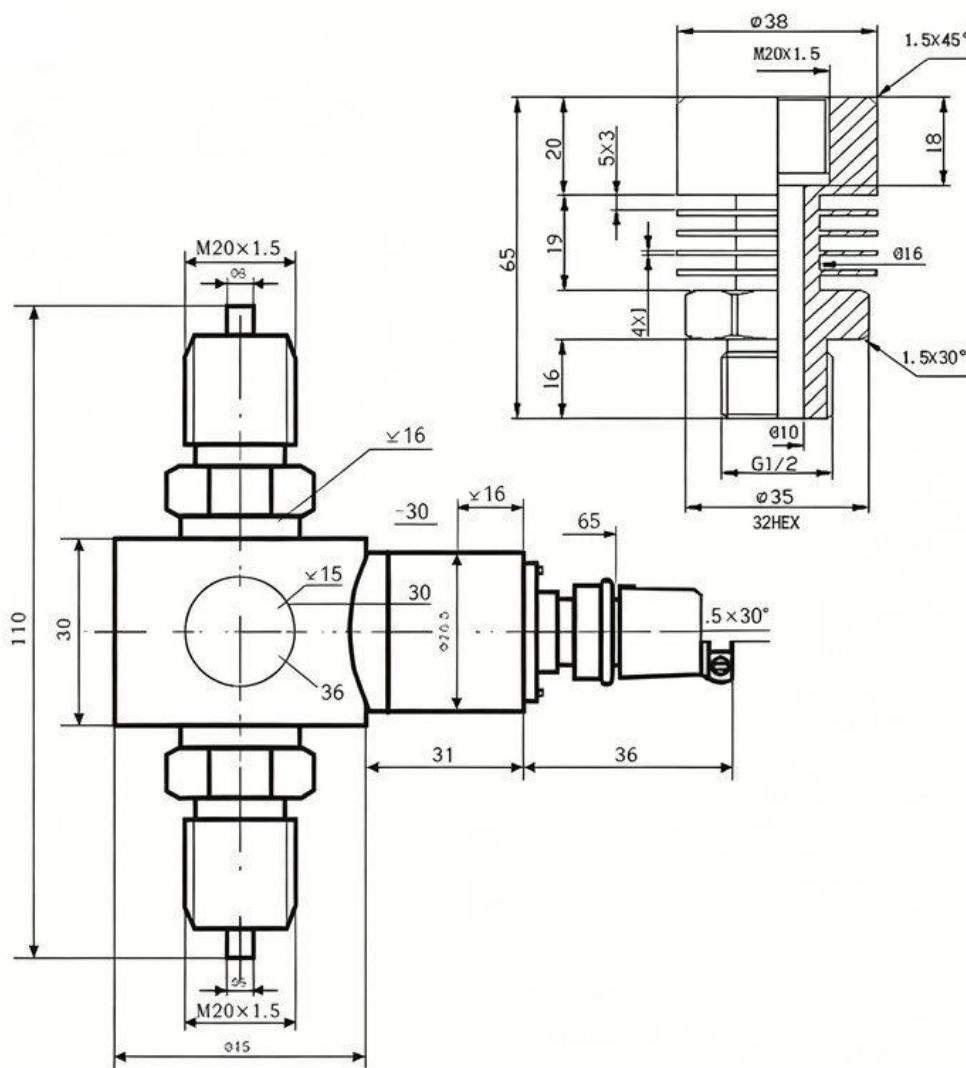
Product Dimensions
