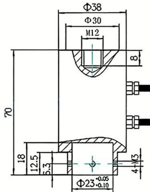
MLC5038F2-SIZE
