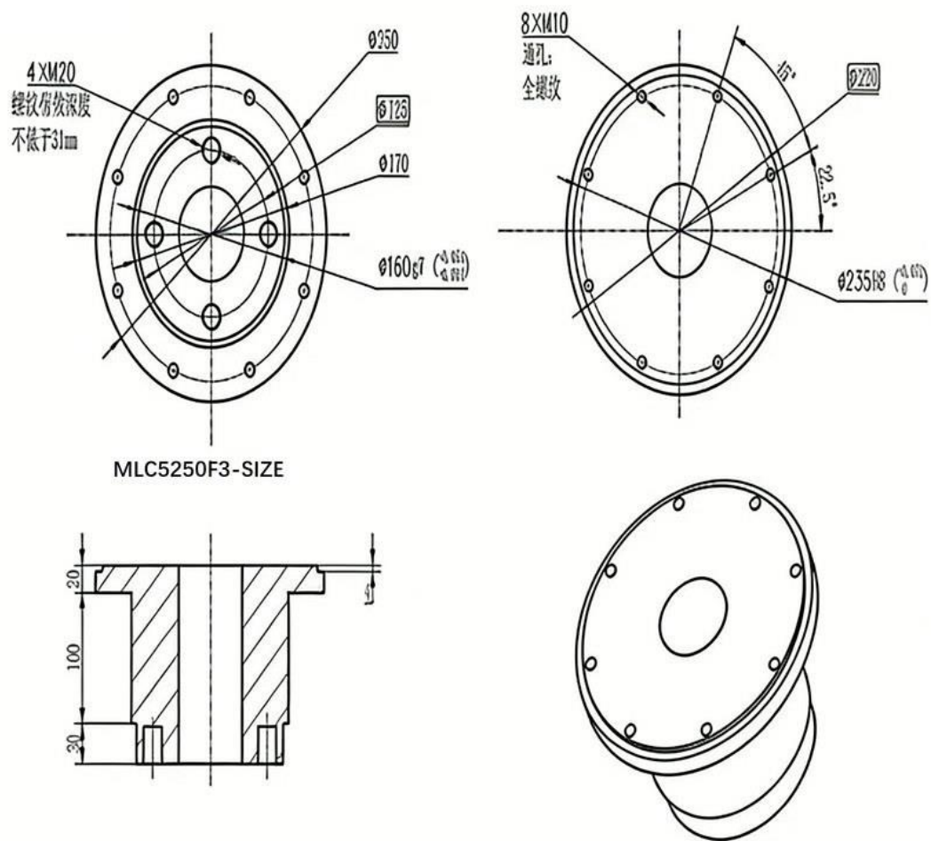
Product Dimensions
