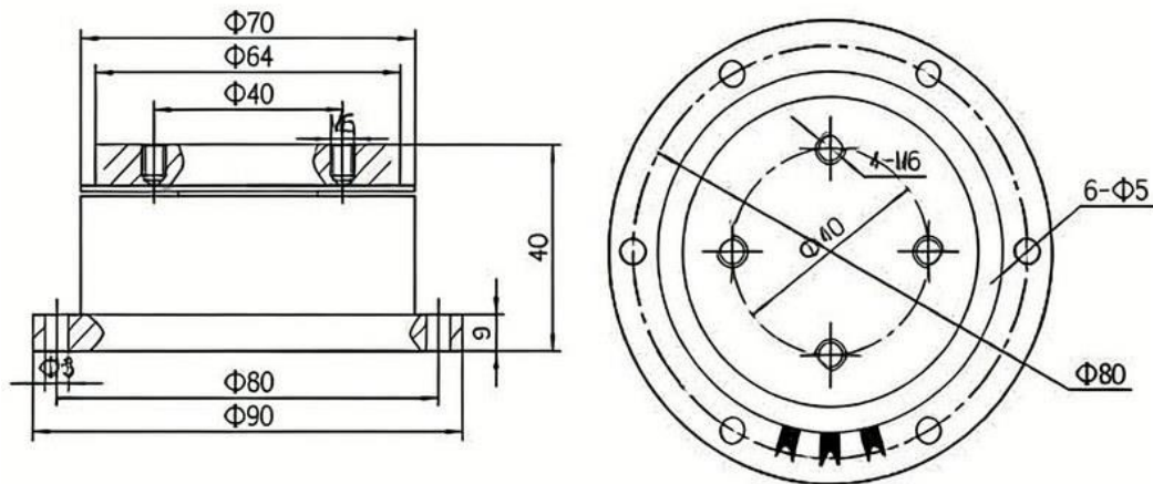
MLC5090F3-SIZE
